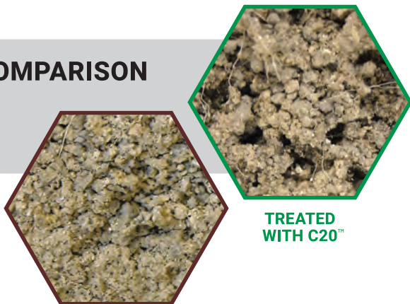
UNTREATED SOIL
